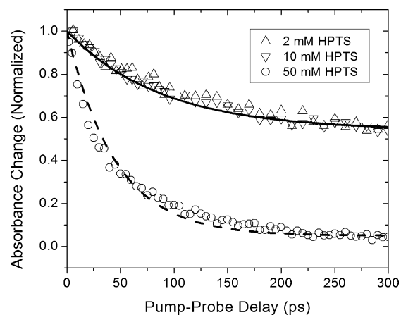
Figure 2. HPTS concentration dependence of the proton continuum decay (HPTS in \text{H}_2\text{O} ). At HPTS concentrations higher than \sim 20 mM self-quenching competes with acid dissociation as a de-excitation channel. At a HPTS concentration of 50 mM, this leads to a complete decay of the continuum signal similar to that observed in previous work. 24
