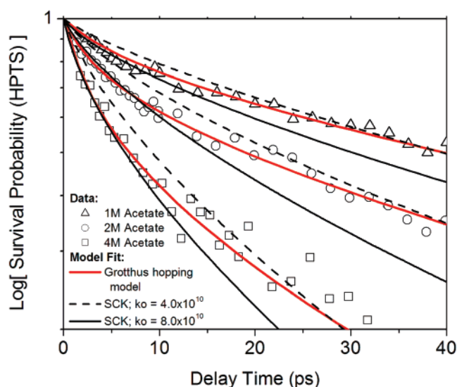
Figure 7. Comparison of Grothuss and SCK models. The decay of the deuteron continuum (HPTS survival probability) for HPTS in \text{D}_2\text{O} at acetate concentrations of 1 M, 2 M, and 4 M are compared with calculations using the Grothuss hopping and SCK models. Two SCK decay curves are shown, one for the on-contact rate parameter k_0 = 4 \times 10^{10} \text{ M}^{-1} \text{ s}^{-1} and one for k_0 = 8 \times 10^{10} \text{ M}^{-1} \text{ s}^{-1} (other SCK model parameters are described in the text). The SCK model is unable to reproduce the strong nonexponentiality of the data over the first 40 ps.
